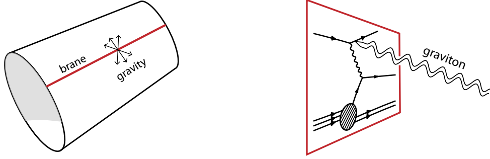
Figure 4: Cartoon pictures of a (3+1) dimensional brane in a compact 5D space. (LEFT) The brane (red line) as a subspace. Gravity propagates in the entire space ‘diluting’ its field lines relative to forces localized on the brane. (RIGHT) SM processes localized on the brane, now with an additional dimension drawn, emitting a graviton into the bulk.
