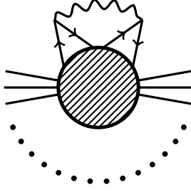
Figure 9: ‘Cat diagram’ adapted from [147]. Despite the silly appearance, the key point is that the photon couples to the electric current J_\mu = e\bar{\Psi}\gamma_\mu\Psi (‘ears’) formed from interactions with fundamental quarks in the strongly coupled sector. The ‘whiskers’ are the pseudo-Goldstone external states when expanding the U(x) field in (4.28). The contribution to the charged meson masses come from the ‘two whisker’ diagram.
