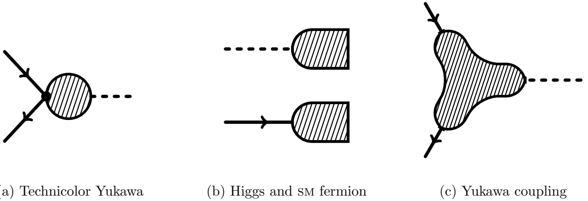
Figure 11: Fermion couplings to the composite sector, represented by shaded blobs. (a): Bilinear coupling of fermions to the composite sector (4.48) lead to ‘technicolor’ types of Yukawa couplings. (b): Partial compositeness scenario. In addition to the Higgs being part of the strong sector, the elementary SM fermions mix linearly with strong sector operators with the same quantum numbers. (c): Yukawa interactions are generated through the strong sector dynamics. Adapted from [155].
