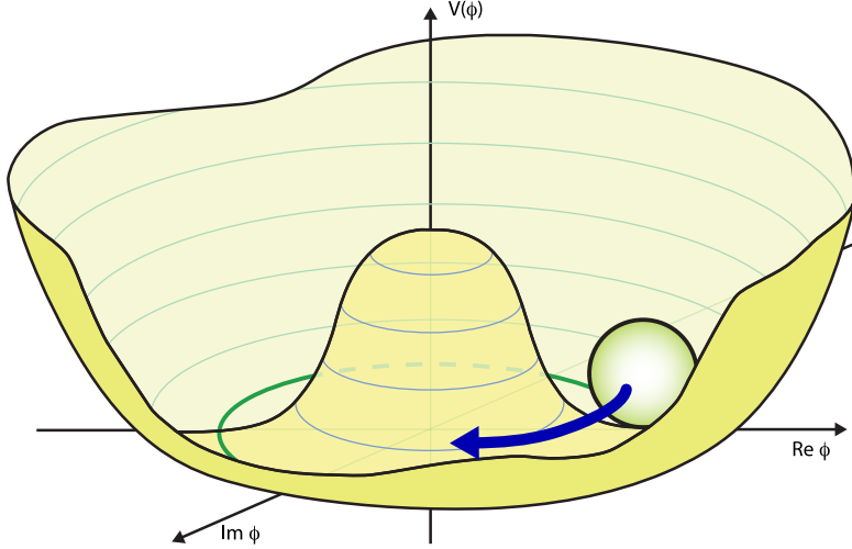
Figure 8: Cartoon of the Goldstone excitation for a ‘Mexican hat’ potential. Image from [143].
