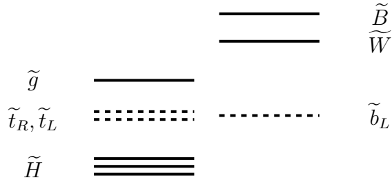
Figure 3: Heuristic picture of a natural SUSY spectrum. All other superpartners are assumed to have masses well above the TeV scale and decouple.
