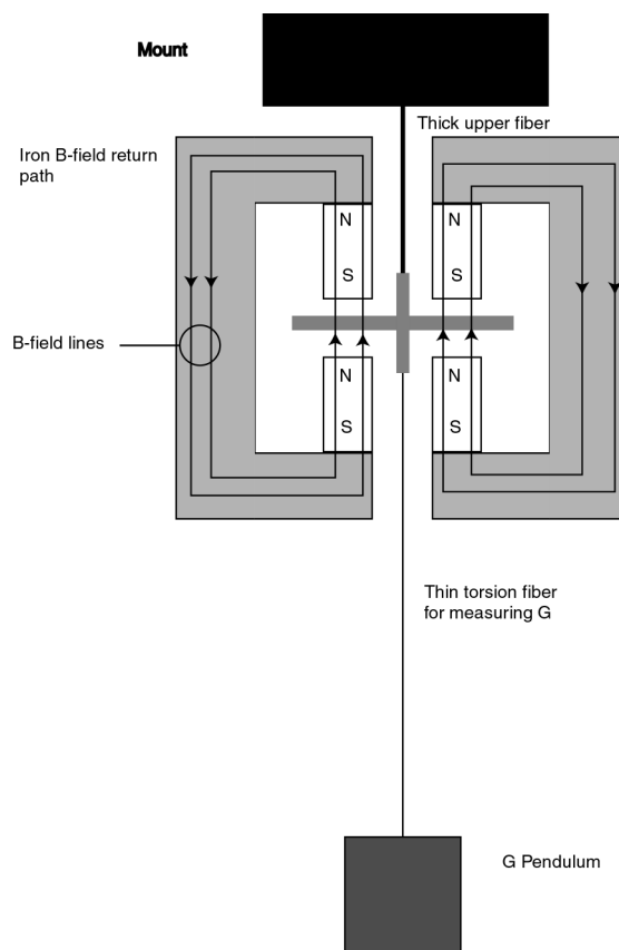
Figure 4.5 Cross Section of an Azimuthally Symmetric Swing Mode Eddy Current Damping Device
