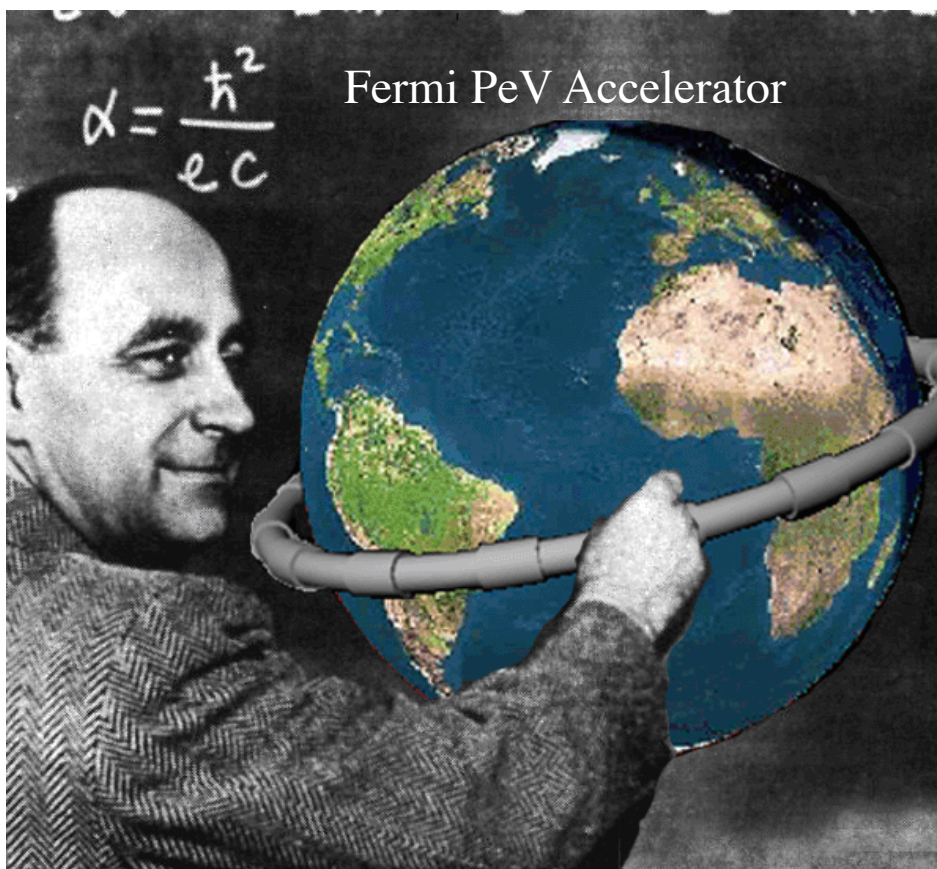
Fig.X.1: Fermi's PeV vision
