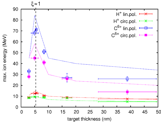
Fig. V.2 Maximum ion cutoff energies as a function of target thickness in the regime of CAIL experiments [30]. Theoretical curves are from the CAIL theory as discussed here [31], [32]. Observed values and theory (CAIL) are in good agreement over a broad parameter range. (from ref. [31]).
