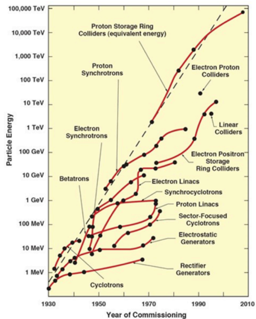
Fig. I.1: Livingston chart (from Ref. [1])
