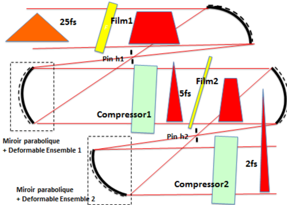
Fig.II.2: Embodiment of a double Thin Film Compressor TFC Thin film "plastic" of 500\mu\text{m} thickness as uniform as possible is set in the near field of PW producing a flat-top beam with the B-integral value ( B ) of about 3-7. The beam propagate through a telescope composed of 2 parabolae, used to adjust finely the B and reduce the laser beam hot spots. Before compression the beam is corrected for the residual wavefront non-uniformity of the beam and the thin film thickness variations. The pulse is compressed using chirped mirrors to 6.4fs. The measurement is performed using a single shot auto-correlator. The same step is repeated in a second compressor with a film of 100\mu\text{m} producing an output of 2 fs, 20J. (After [37])
