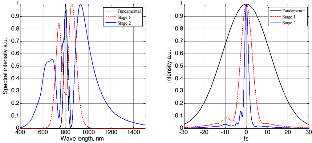
Fig. II.4: Successive spectra and pulse durations corresponding to the laser output, after the first stage and second stage. After the first stage the pulse length is 6.4fs, and after the second stage the pulse is shrunk to 2.1fs (after [37])
