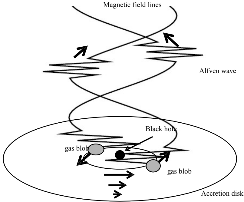
Fig. VII.1: MRI (magneto-rotational instability) triggers disk disturbance. [179] This triggers gas blobs to accrete toward the central black hole, which launches massive excitation of a pulse of magnetic disturbances in the jet. [176].
