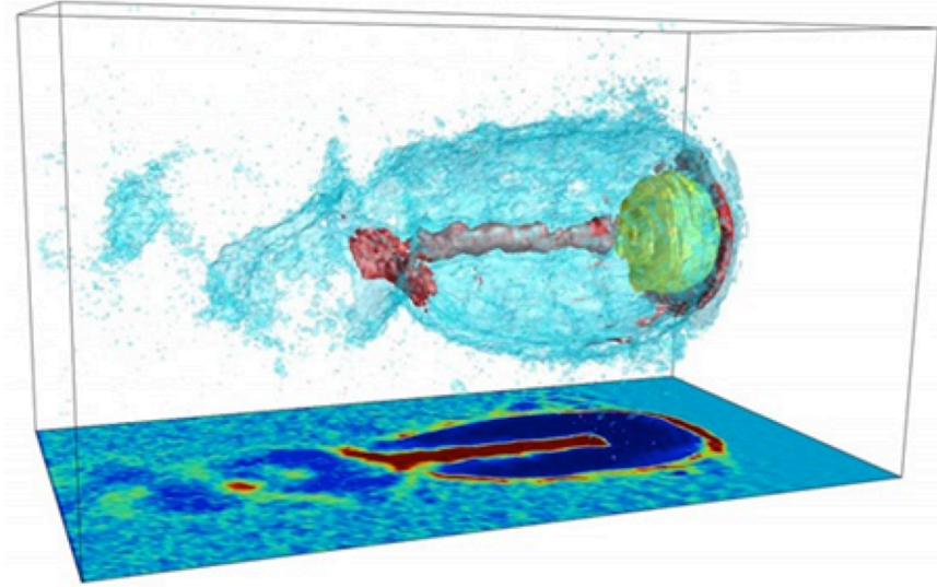
Fig. III.1 Electron density distribution of a laser wake in the bubble regime, computed with the 3D PIC simulation. From [90]
