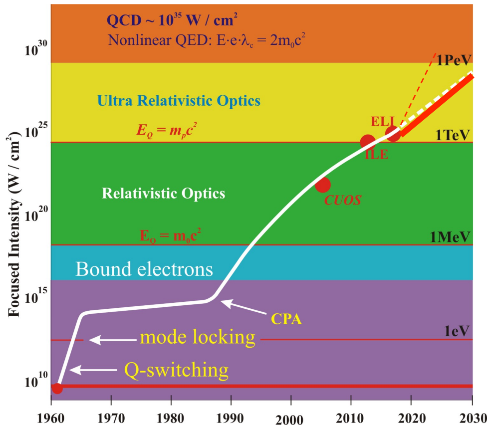
Fig.X.2: The laser intensity in years. A shortcut (dotted red line) toward EW and ultrahigh intensities. (After [142] with revisions).
