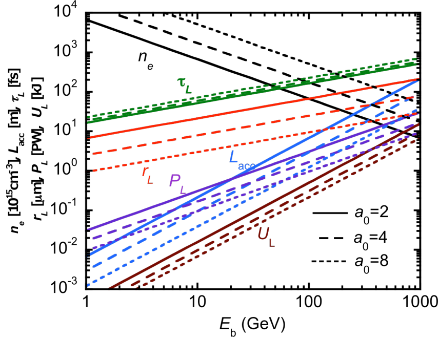
Fig. III.3 Parameters for the self-guided case in the bubble regime with a_0 = 2 (solid line), a_0 = 4 (dashed line), a_0 = 8 (dotted line), \alpha_c = 0.9 for \lambda_L = 351\text{nm} : operating plasma density n_e [ 10^{15}\text{cm}^{-3} ], accelerator length L_{acc} \cong L_{dp} [m], required pulse duration \tau_L [fs], matched spot radius r_L [ \mu\text{m} ], matched peak power P_L [PW] and required pulse energy U_L [kJ], respectively, as a function of electron beam energy E_b [GeV].
