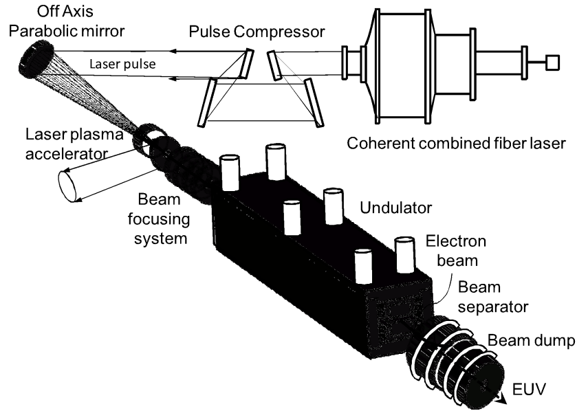
Fig. VIII.1 A schematic illustration for the EUV light source based on a compact Free Electron Laser driven by a fibre laser-based [40] plasma accelerator.
