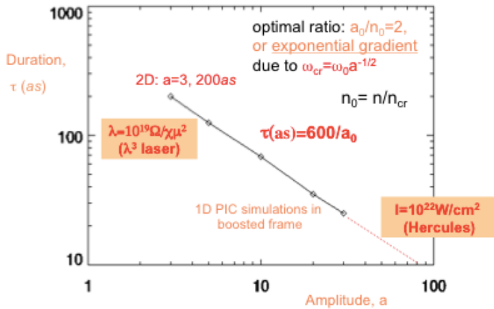
Fig.II.6 Pulse duration as function of a_0 , the normalized vector potential. The expression of the pulse duration is derived to be 600as / a_0 . For a_0 of the order of 1000, pulse duration of 600zs could be achieved. (after [43])
