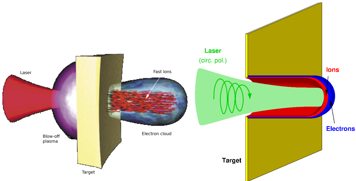
Fig. I.3: The Comparison of the TNSA laser-target interaction and the CAIL one. In the TNSA (left), the target remains unmoved, behind which a sheath is formed and ion acceleration is limited over this sheath. When the target is sufficiently thin (right), some portion of the target may commove with the ponderomotively accelerated electron layer. This achieves partial coherence of ion motion behind the electron sheet. (from ref. [31]).
