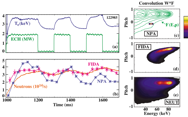
FIG. 7. (Color online) Time evolution of (a) central electron temperature and ECH power and (b) FIDA, NPA, and neutron signals in a DIII-D discharge (Ref. 11) with 2.5 MW of injected beam power from the co-tangential sources. The FIDA signal is integrated over wavelengths corresponding to energy along the line-of-sight of 40–50 keV and is divided by the estimated neutral density at the position of the measurement. The NPA signal is from active charge exchange at the same location as the FIDA channel ( R \approx 196 cm) and is corrected for changes in neutral density and for attenuation of the escaping neutrals. (c) Contours of the fast-ion distribution function computed by the TRANSP NUBEAM code for this condition. The NPA measures a localized region in velocity space. Product of the weight function W and the distribution function F for (d) the FIDA measurement and (e) the beam-plasma neutron measurement. (c)–(e) adapted and reprinted with permission from W. W. Heidbrink et al. , Plasma Phys. Controlled Fusion 49 , 1457 (2007). Copyright © 2007, IOP Publishing Ltd.
