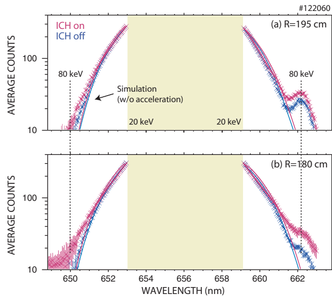
Figure 4. Average FIDA spectra (symbols) with and without ICH for the channels at (a) R = 195 cm and (b) 180 cm in the discharge shown in figure 3 between 2250–2500 ms and 1700–2000 ms, respectively. The solid lines show the spectra predicted by the FIDA simulation code for the TRANSP fast-ion distribution function calculated in the absence of ICH acceleration. The dotted vertical lines indicate the wavelengths that correspond to E_\lambda = 80 keV. The FIDA simulation only treated the portion of the fast-ion distribution function with energies above 20 keV. Although the most prominent impurity lines have already been fitted and removed from the spectra [30], an impurity line at 662.15 nm still appears.
