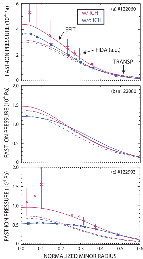
Figure 6. Fast-ion pressure inferred from equilibrium analysis (solid line) with and without ICH versus normalized minor radius \rho . (a) The fourth harmonic discharge shown in figure 3 at 2285 and 2065 ms. (b) A high-density fourth harmonic discharge at 4450 and 2670 ms. (c) The fifth harmonic discharge shown in figure 5 at 2445 and 1965 ms. The dashed lines are the fast-ion pressure predicted by TRANSP for classical behavior with ICH acceleration ignored. The symbols represent FIDA density data that are averaged over \sim 200 ms and E_\lambda = 45\text{--}75 keV; the data are normalized to agree with the pressure profile without ICH.
