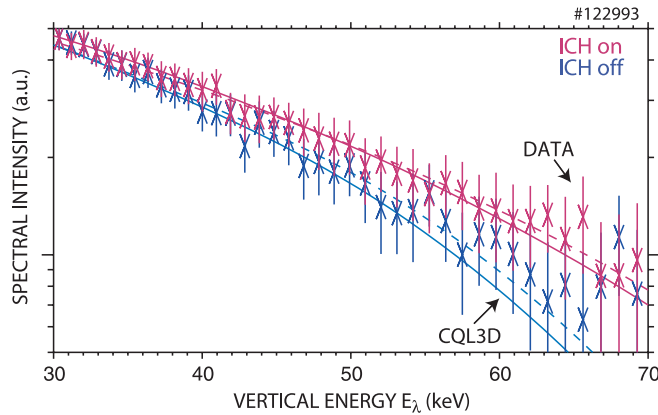
Figure 10. Measured (symbols) and calculated (curves) FIDA spectra with (2200–2700 ms) and without (1500–2000 ms) ICH in the fifth-harmonic discharge shown in figure 5. The CQL3D predictions are for the 180 cm channel (—) and for the 176 cm channel (- - -); the data are from the 180 cm channel.
