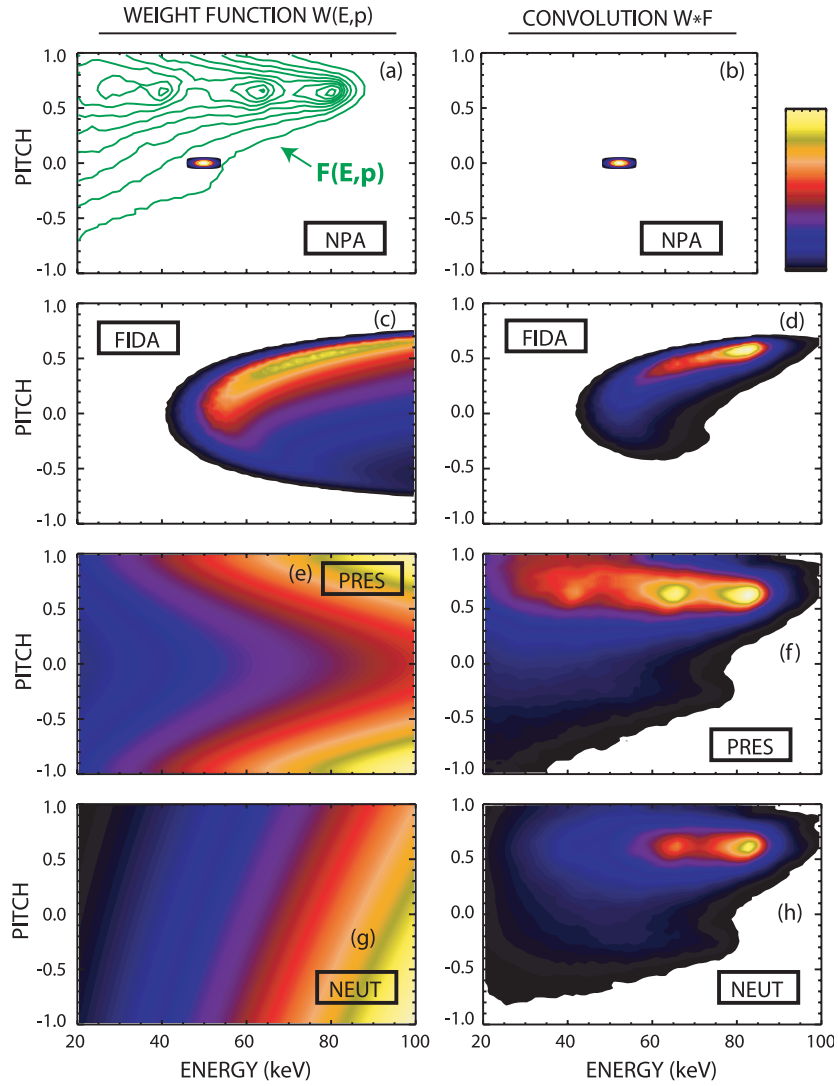
Figure 2. Contour plots of the velocity-space weight functions (left column) for the NPA, FIDA, p_f , and neutron diagnostics for discharge #122060 before the ICH. The bar graph in the upper right figure shows the linear color scale in normalized units. The upper left graph also shows the fast-ion distribution function F(E, p) calculated by TRANSP at the location of the 180 cm FIDA channel. The right column shows contour plots of the product of the weight function with the TRANSP distribution function for the four fast-ion diagnostics. The FIDA graphs use the calculated injected neutral densities at 180 cm (full : half : third of 57% : 26% : 17%), include an approximate treatment of the instrumental resolution (Gaussian spread with \sigma = 0.21 nm), and assume E_\lambda = 50 keV. The neutron weight function is for beam-plasma reactions only and employs the measured ion temperature ( 5.0 keV) and toroidal rotation ( 2.1 \times 10^7 cm s ^{-1} ). The weight function is negligible in the white regions.
