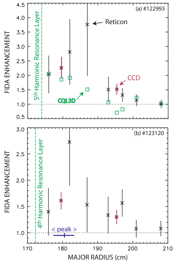
Figure 11. Relative change in FIDA density during ICH versus major radius for central (a) fifth harmonic heating and (b) fourth harmonic heating. The data from the dedicated diagnostic (*) are integrated over E_\lambda = 48\text{--}77 keV and the data from the diagnostic that uses Reticon detectors (x) are integrated over wavelengths that correspond to E_\lambda = 45\text{--}65 keV. The square symbols are the theoretical predictions of the CQL3D code. The dashed lines represent the nominal resonance layer without fast-wave Doppler shift corrections. In the lower figure, the average and standard deviation of the peak location for five discharges similar to #123120 are indicated by the symbol near 180 cm.
