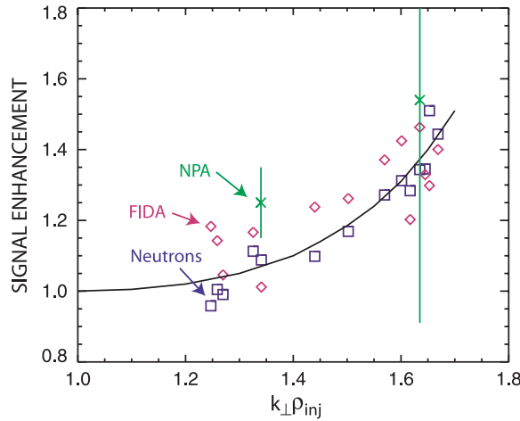
Figure 9. Signal enhancement during ICH for the neutron ( \square ), FIDA ( \diamond ), and NPA ( \times ) diagnostics versus the normalized gyroradius of the injected beam ions for all of the fourth harmonic discharges with quiet MHD and > 0.5 MW of 60 MHz ICH in the database. The abscissa employs the approximation k_{\perp} \simeq \omega_{\text{RF}}/v_A , with the Alfvén speed evaluated using the line averaged electron density and nominal toroidal field. The solid curve is taken from [11]. The FIDA data are from the R = 180 cm channel and are averaged over E_{\lambda} = 55\text{--}80 keV. The NPA points are the mean and standard deviation of several discharges with the analyser set to measure neutrals of 50 keV.
