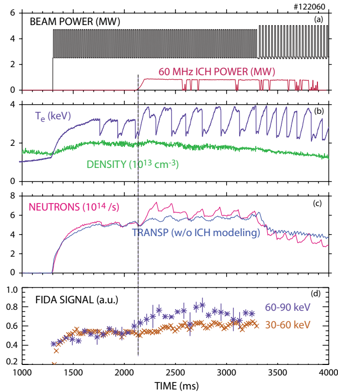
Figure 3. Time evolution of (a) the injected neutral beam and coupled ICH power, (b) the central electron temperature and the line-average electron density, (c) the measured neutron rate and the classically expected rate in the absence of ion cyclotron acceleration and (d) the FIDA signal in two spectral bands. The more tangential left beams are injected from 1300 to 3300 ms, while more perpendicular right beams are injected after 3300 ms. For the FIDA data, the ‘30–60 keV’ signal represents E_\lambda between 30 and 60 keV (wavelengths between 650.8–652.4 and 659.8–661.3 nm) and the ‘60–90 keV’ signal integrates wavelengths between 649.6–650.8 and 661.3–662.6 nm. The radial position of the FIDA channel is centered at R = 195.4 cm. B_T = 1.92 T; I_p = 1.0 MA.
