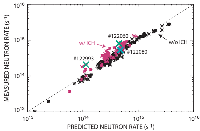
Figure 7. Measured neutron rate versus the prediction of a zero-dimensional model [34] for quiet plasmas with over 0.75 MW of ICH power (red) and with less than 0.5 MW of ICH (black). The three discharges selected for detailed analysis are indicated. None of the discharges have tearing or Alfvén modes.
