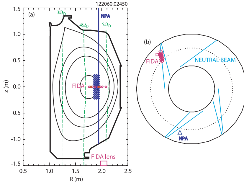
Figure 1. (a) Elevation of the DIII-D vacuum vessel, showing the separatrix and the q = 1, 2 and 3 surfaces (solid black curves), the locations where \omega_{RF} equals the third, fourth and fifth deuterium cyclotron harmonic (dashed green curves), the NPA sightline (thick blue vertical line), and the midplane locations of the FIDA Reticon (diamond) and CCD (solid triangle) chords. The hashed region represents the approximate vertical extent of the heating beam that produces the FIDA and NPA signals. The square indicates the approximate location of the FIDA collection optics. (b) Plan view of the vessel, showing the toroidal location of the FIDA and NPA diagnostics and the centerlines of the various left and right beams. The dotted line represents the magnetic axis.
