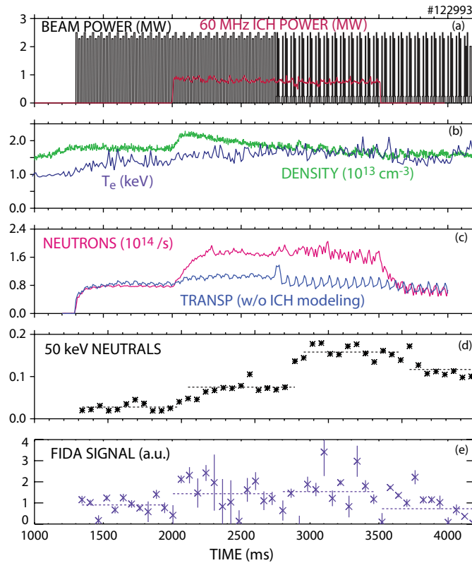
Figure 5. Time evolution of (a) the injected neutral beam and coupled ICH power, (b) the central electron temperature and the line-average electron density, (c) the measured neutron rate and the classically expected rate in the absence of ion cyclotron acceleration, (d) the active charge-exchange signal from the vertical NPA (with neutral density and neutral attenuation corrections) and (e) the FIDA density. The more tangential left beams are injected from 1300 to 2750 ms, while an equal mixture of left and right beams are injected from 2750 to 4150 ms. The FIDA data are integrated over wavelengths between 649.6–650.8 and 661.3–662.6 nm for the channel that is centered at R = 179.6 cm. The dotted lines show the average values of the (d) NPA and (e) FIDA data over the four time periods: left beams and no ICH, left beams with ICH, mixed beams with ICH, mixed beams no ICH. B_T = 1.53 T; I_p = 1.0 MA.
