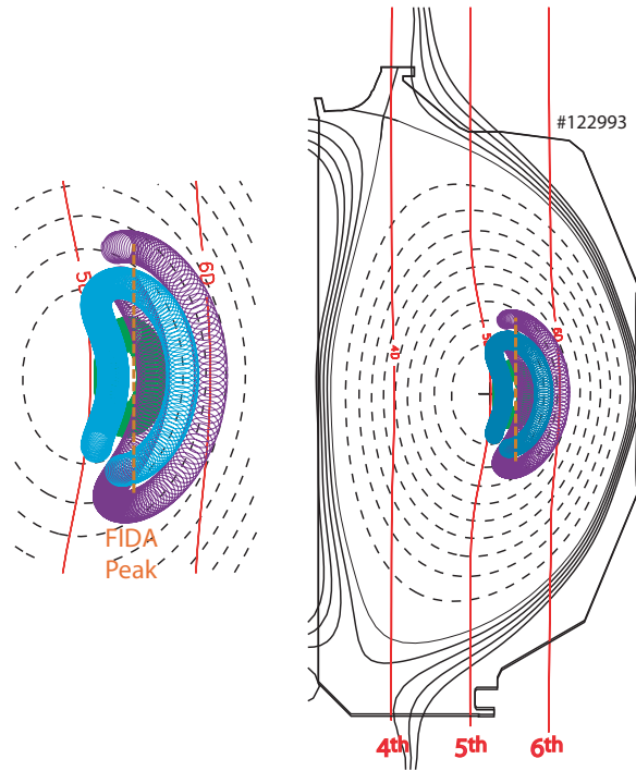
Figure 12. Elevation of DIII-D for the discharge shown in figure 5, showing the projection of representative orbits that have values of v_z that contribute strongly to the observed enhancement of the FIDA signal and are launched from the radial location of the peak of the FIDA enhancement. The dashed lines represent flux surfaces and the solid lines represent the nominal resonance layers (neglecting Doppler shifts).
