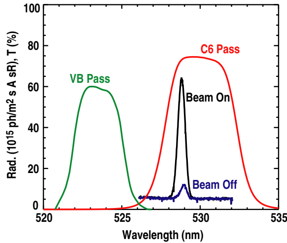
Figure 11. Spectrum from discharge 135847 showing C VI charge exchange line at 529.05 nm measured using CER spectrometer with ('beam on') and without ('beam off') 30L neutral beam on. Spectrometer intersects 30L beam at (R, z) = (2.08, 0.00) . Spectrum baseline level is primarily due to VB. Transmission functions of bandpass filters used for C VI CER and VB measurements are also shown.
