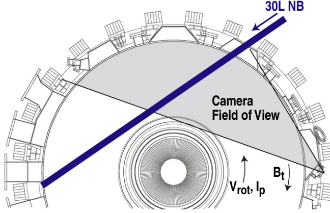
Figure 1. Plan view of DIII-D tokamak showing the camera viewing region in gray. Arrows indicate direction of toroidal field ( B_t ), plasma current ( I_p ), toroidal rotation ( v_{\text{rot}} ) and neutral beam injection. The 1/e width of the 30L neutral beam is approximately to scale.
