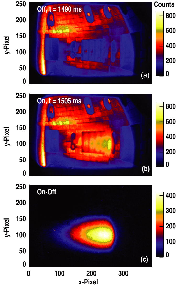
Figure 3. D_\alpha imaging data from DIII-D discharge 135851 showing (a) 30L beam off, (b) 30L beam on, (c) panel (b) through panel (a). Camera sampling rate was 900 frames s^{-1} and exposure time was 1.1 ms. Approximately the top ten and bottom 30 rows of pixels are dark due to mechanical clipping of the FOV. ‘Counts’ are out of 4096 set by camera dynamic range of 12-bits.
